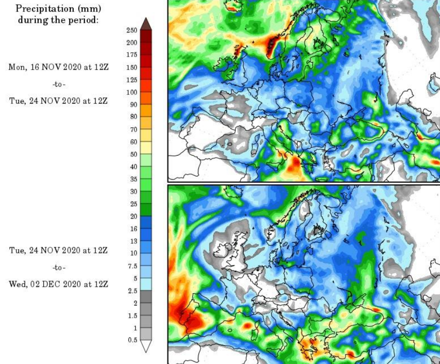
Precipitation Forecasts
