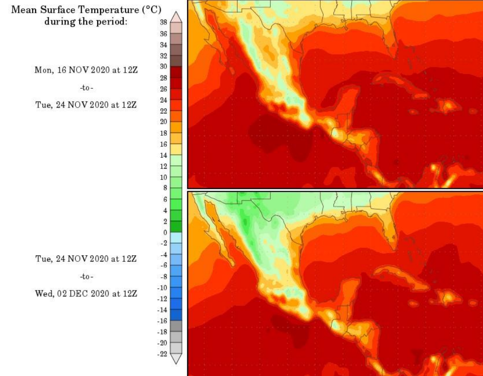
Temperature Forecasts
