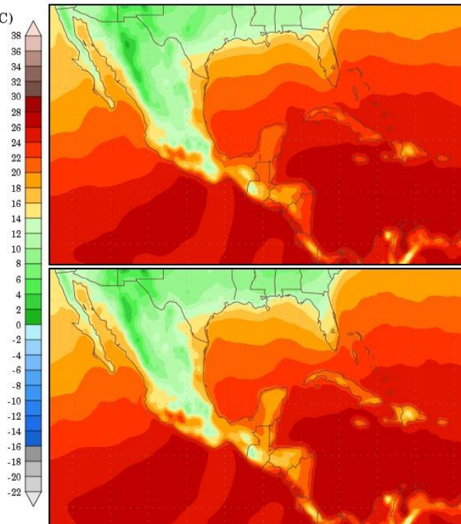
Temperature Forecasts
