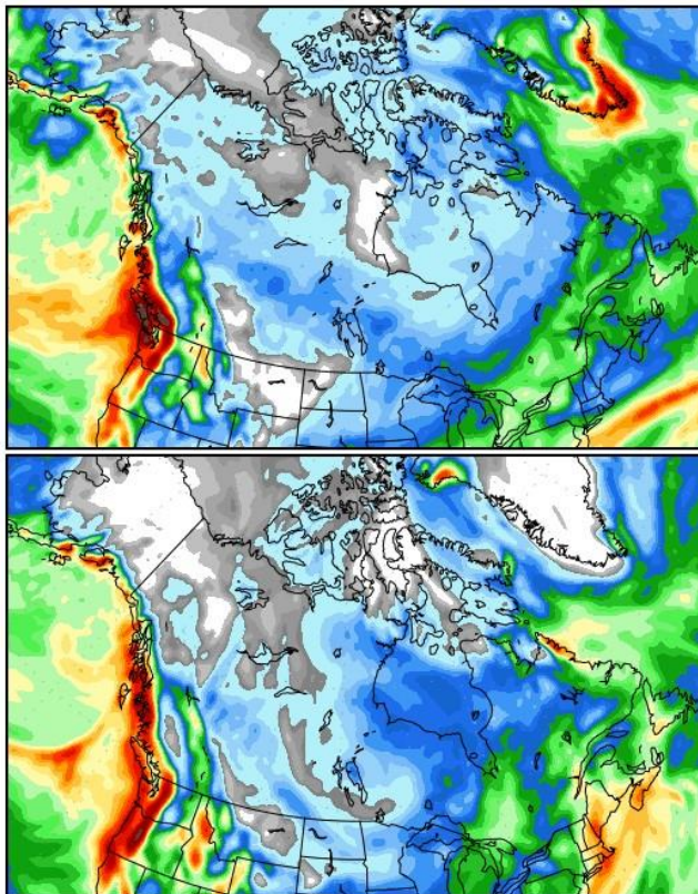
Precipitation Forecasts
