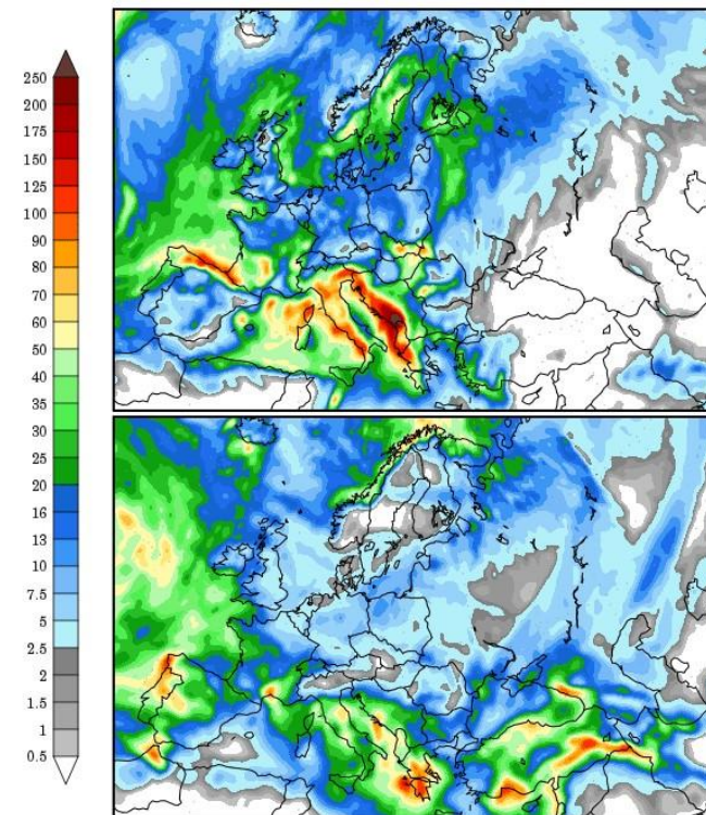
Precipitation Forecasts
