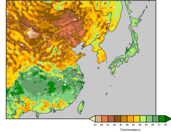
Initial Soil Moisture Liquid Water in top 2 meters of soil Valid time: Mon, 14 DEC 2020 at 00Z
