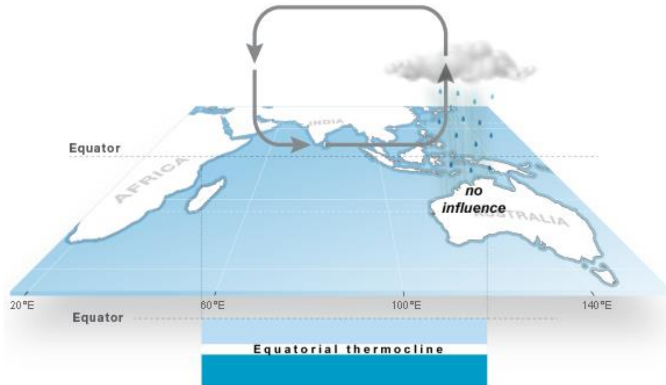
Indian Ocean Dipole (IOD): Neutral phase
