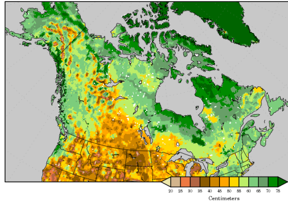
Initial Soil Moisture Liquid Water in top 2 meters of soil Valid time: Mon, 14 DEC 2020 at 00Z
