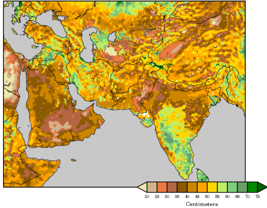
Initial Soil Moisture Liquid Water in top 2 meters of soil Valid time: Mon, 28 DEC 2020 at 00Z
