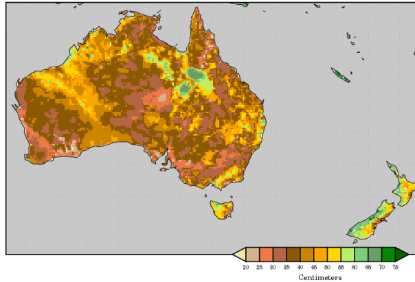
Initial Soil Moisture Liquid Water in top 2 meters of soil Valid time: Mon, 14 DEC 2020 at 00Z
