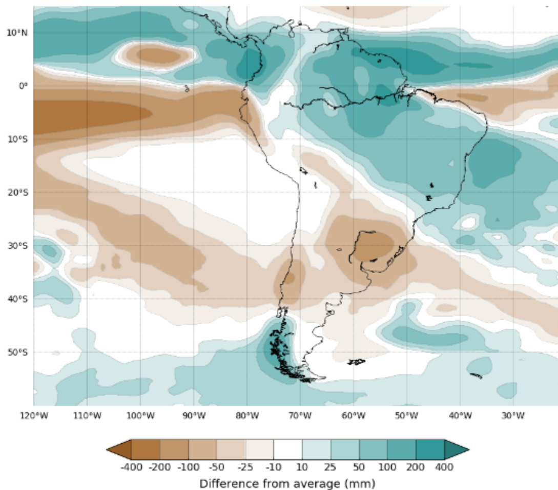
Difference from average rainfall forecast for March to May 2022
