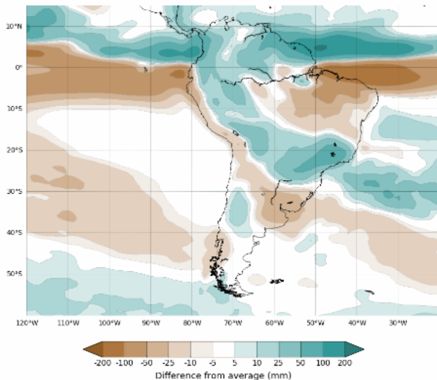
Difference from average rainfall forecast for February 2022
