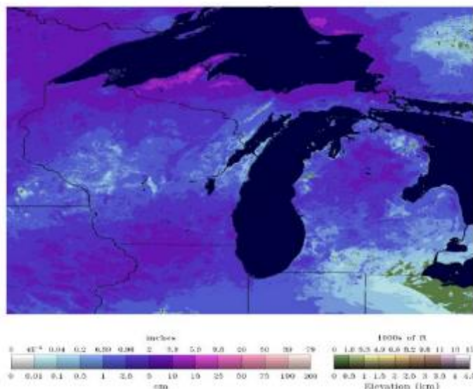
Snow Water Equivalent 2021-01-31 06 UTC
