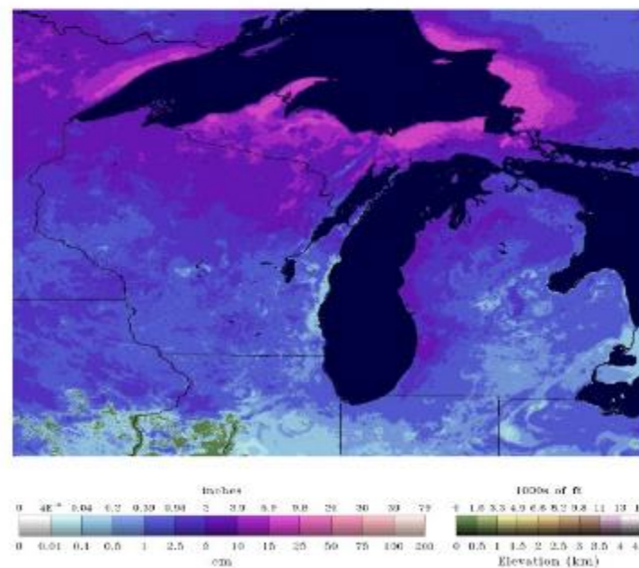
Snow Water Equivalent 2022-01-31 06 UTC
