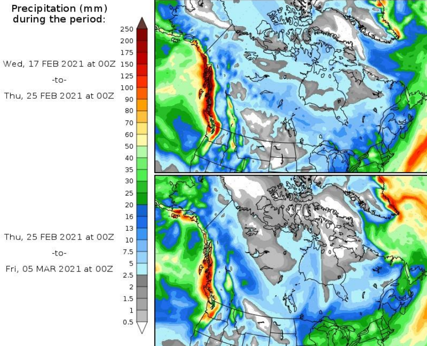
Precipitation Forecasts
