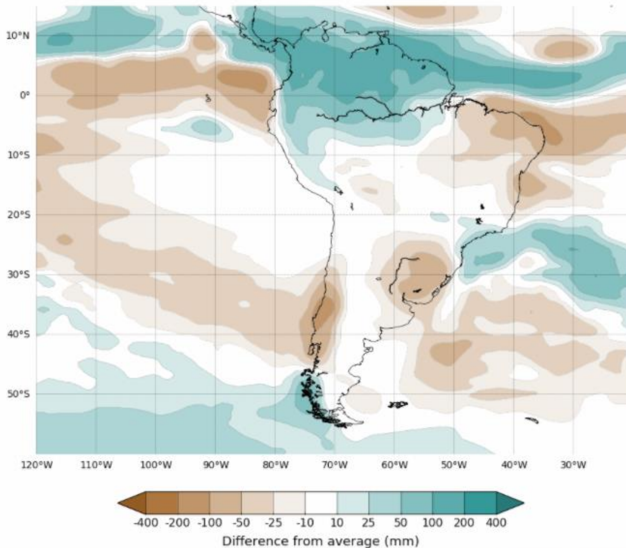
Difference from average rainfall forecast for April to June 2021
