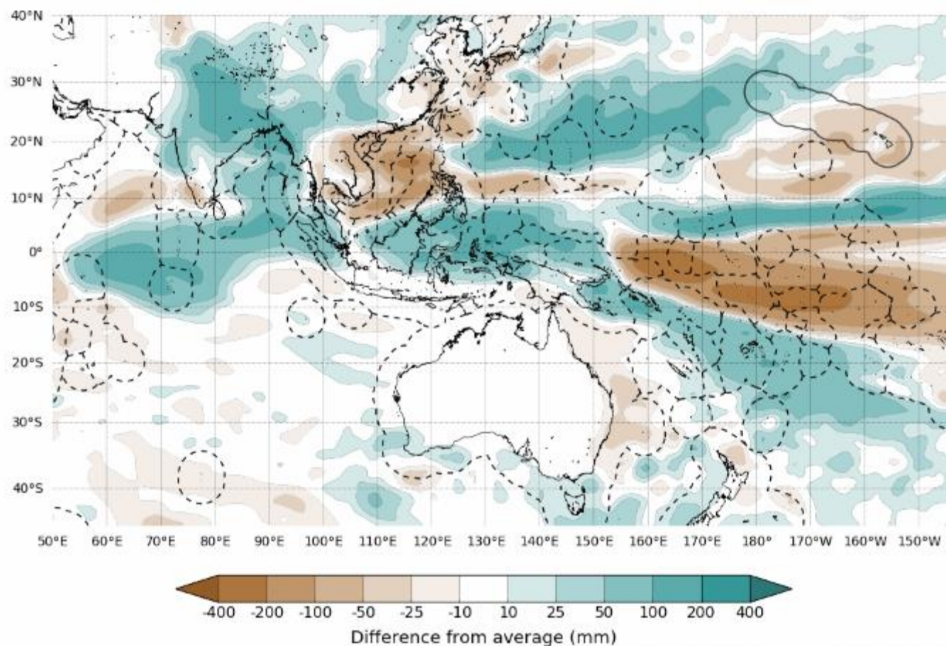
Difference from average rainfall forecast for June to August 2021
