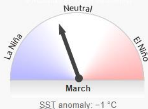
Average of international model outlooks for NINO3.4
