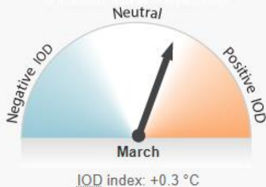
Average of international model outlooks for the Indian Ocean Dipole (IOD)
