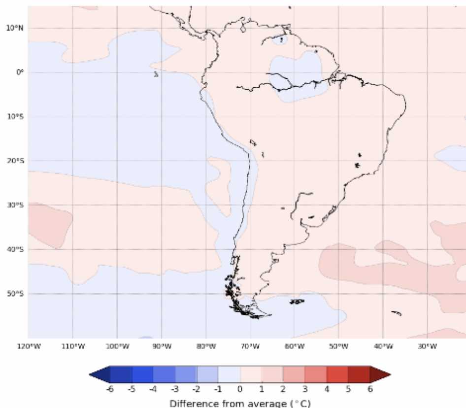
Difference from average mean minimum temperature forecast for February to April 2022
