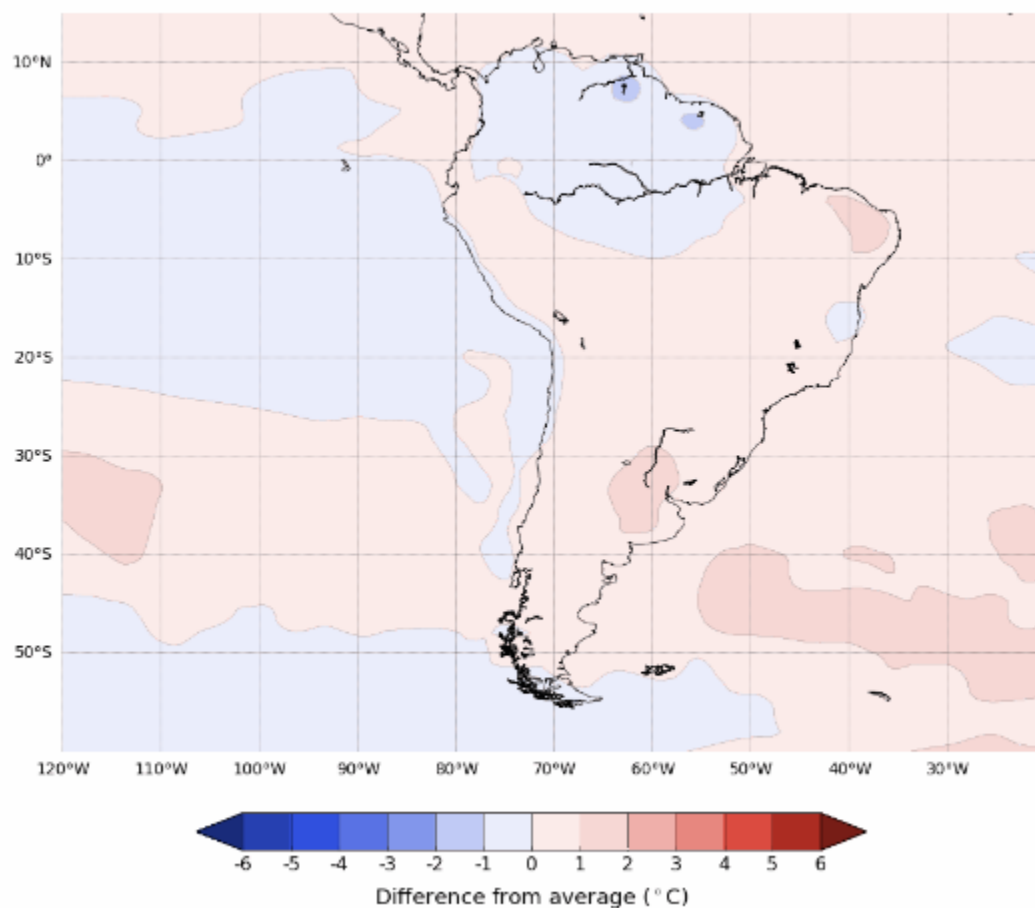
Difference from average mean maximum temperature forecast for February to April 2022
