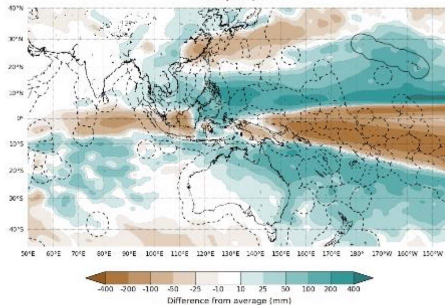
Difference from average rainfall forecast for February to April 2022
