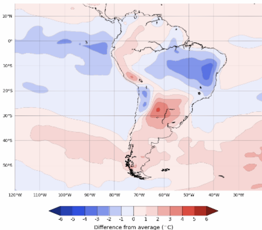
Difference from average mean maximum temperature forecast for 25 to 31 December 2021
