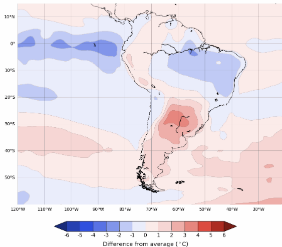
Difference from average mean maximum temperature forecast for 1 to 7 January 2022
