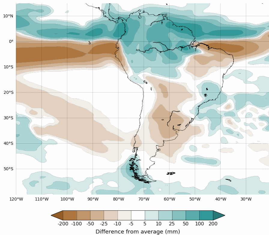
Difference from average rainfall forecast for March 2022
