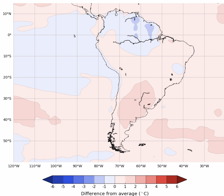
Difference from average mean maximum temperature forecast for March to May 2022
