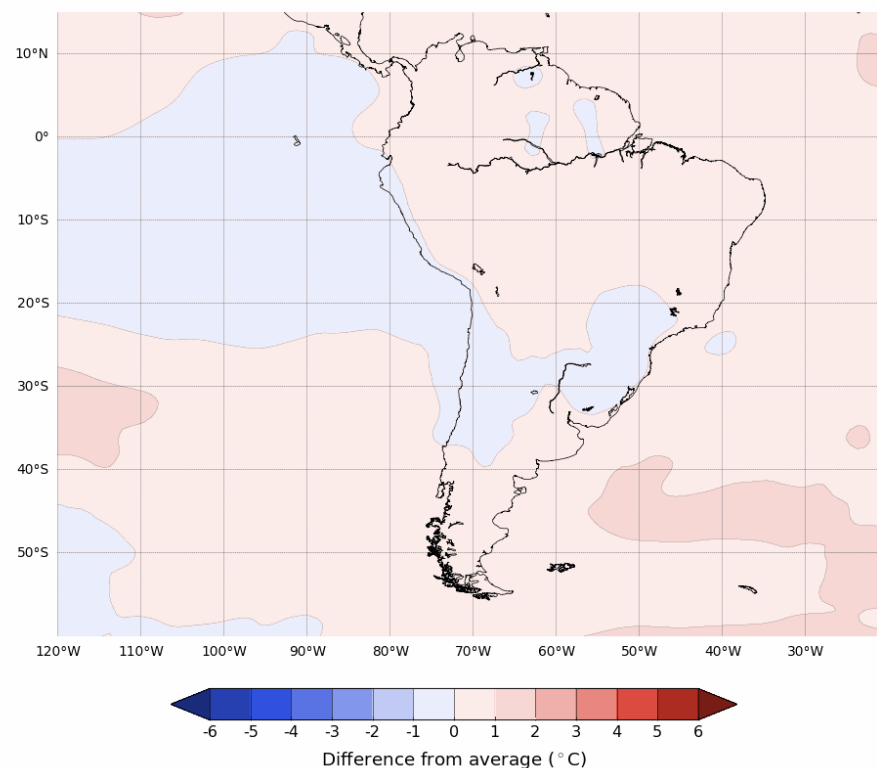
Difference from average mean minimum temperature forecast for April to June 2022
