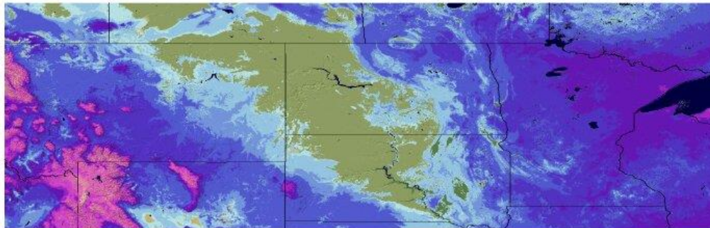
Snow Water Equivalent 2021-02-16 06 UTC
