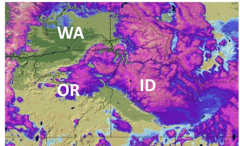
Snow Water Equivalent 2022-02-18 06 UTC
