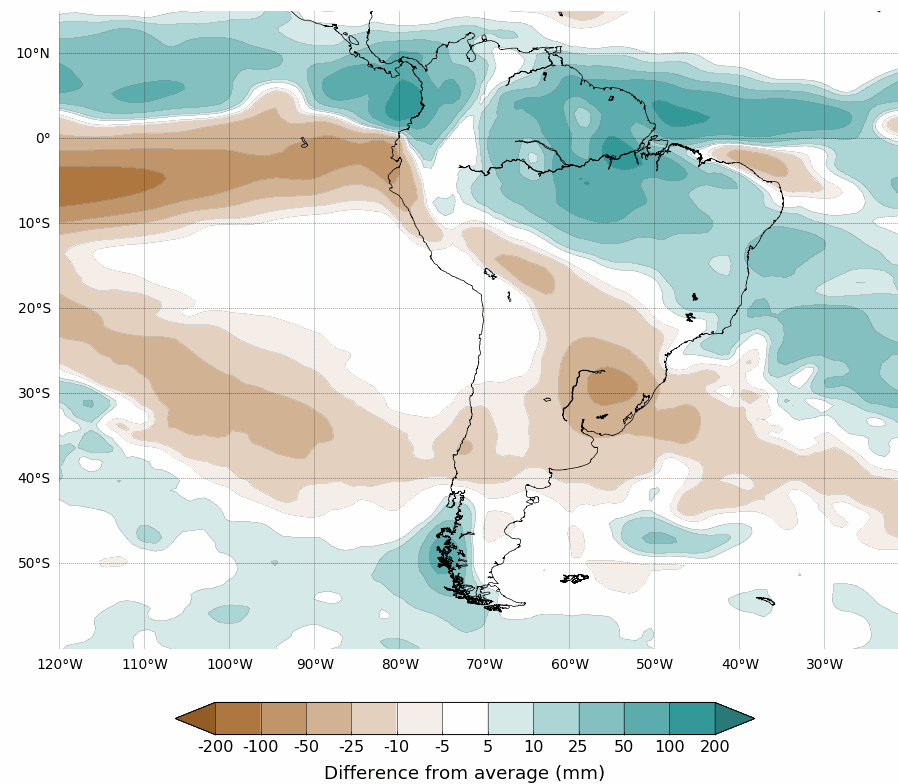
Difference from average rainfall forecast for April 2022
