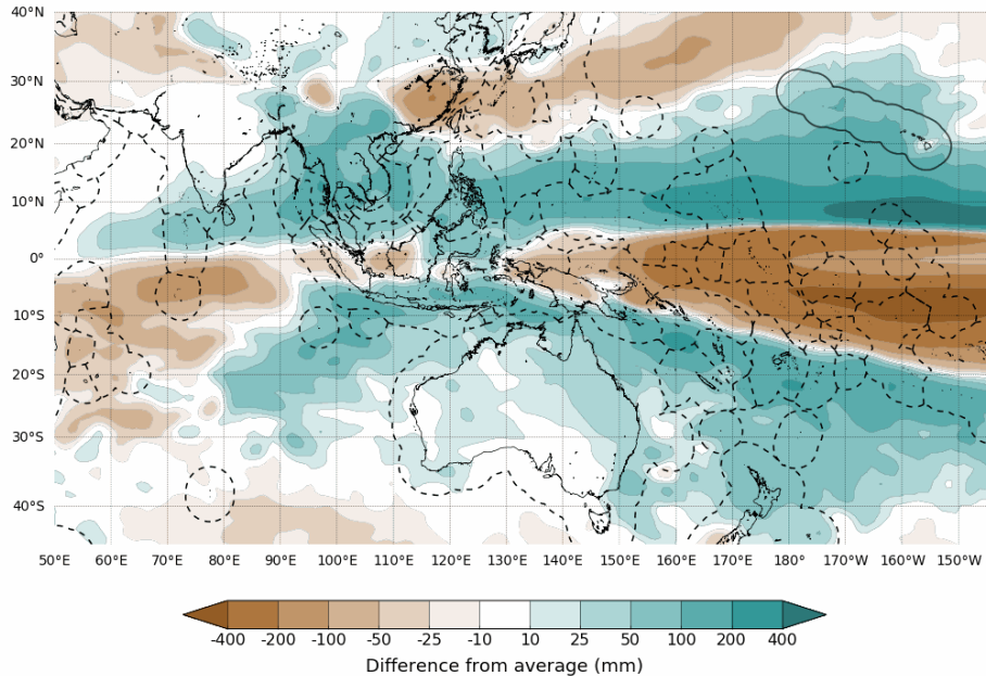
Difference from average rainfall forecast for March to May 2022
