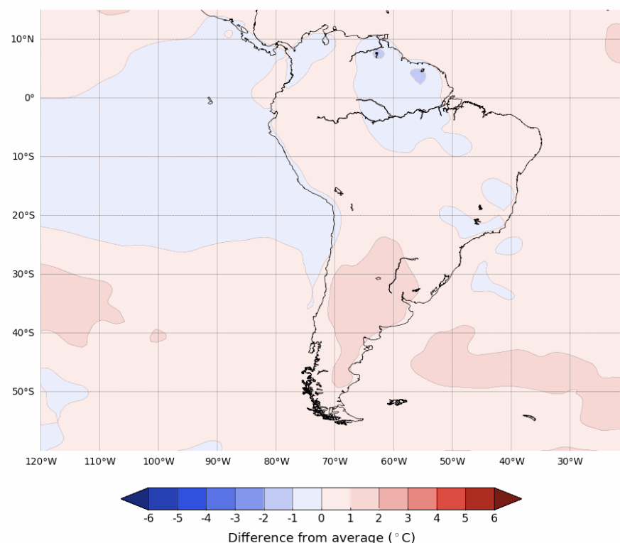
Difference from average mean maximum temperature forecast for April to June 2022
