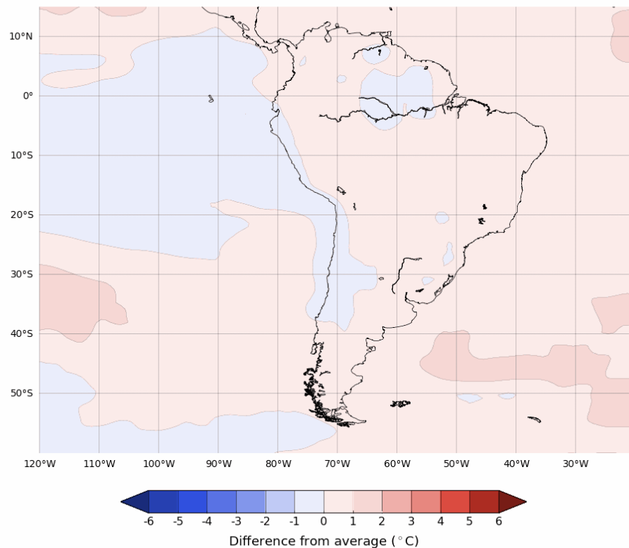
Difference from average mean minimum temperature forecast for March to May 2022
