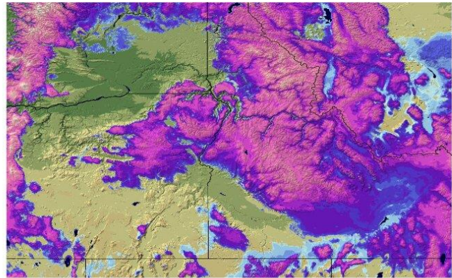
Snow Water Equivalent 2022-02-18 06 UTC
