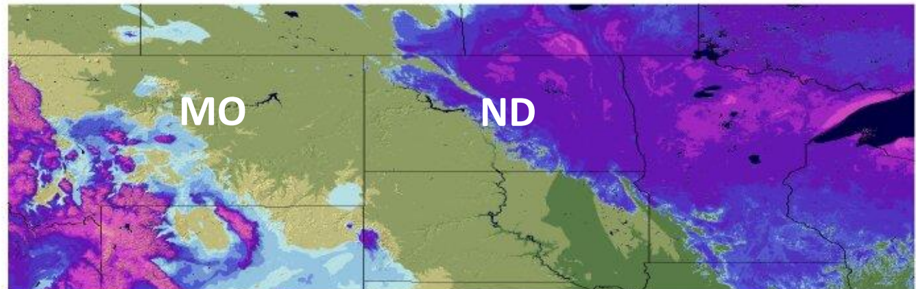
Snow Water Equivalent 2022-02-16 06 UTC
