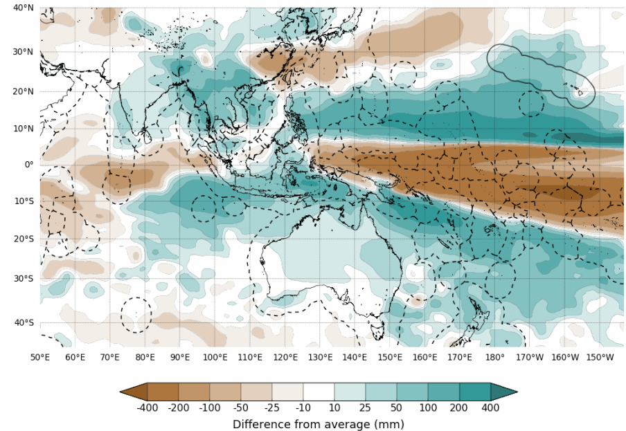
Difference from average rainfall forecast for April to June 2022
